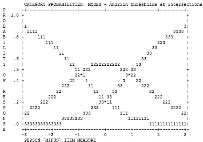
Figura 1. Category Probabilities: Modes - Andrich thresholds at intersections
