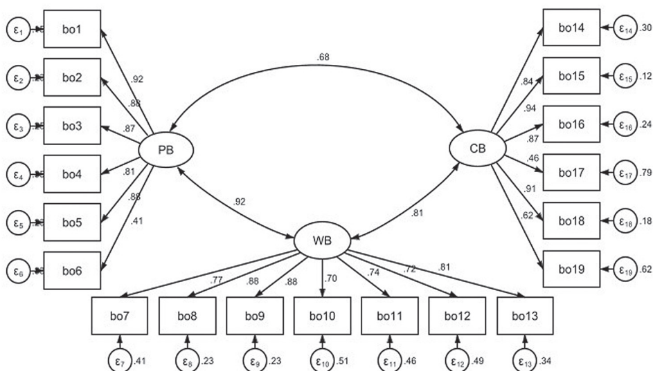
Figura 1. CFA for the 3-correlated factor model
