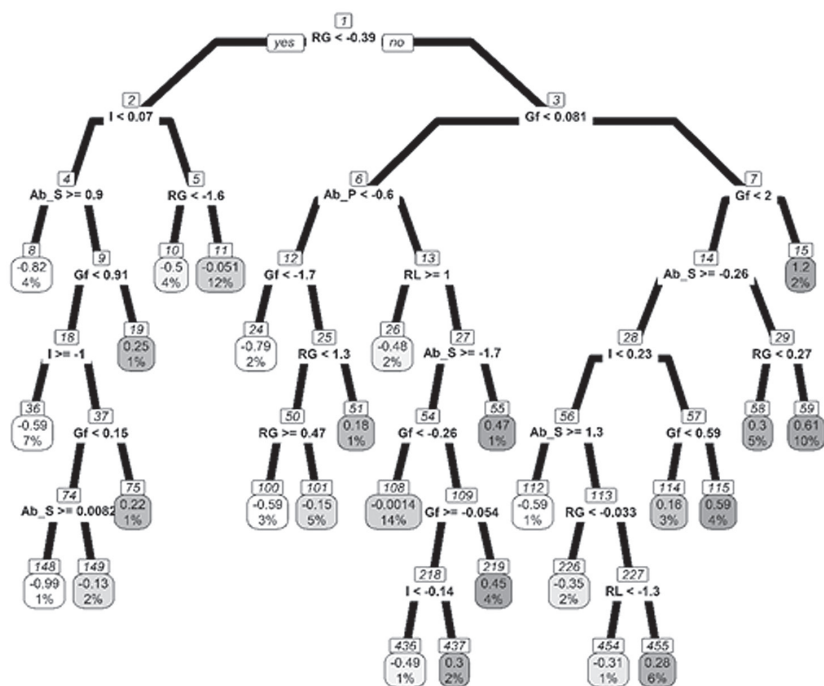
Figure 1. Pruned Tree
